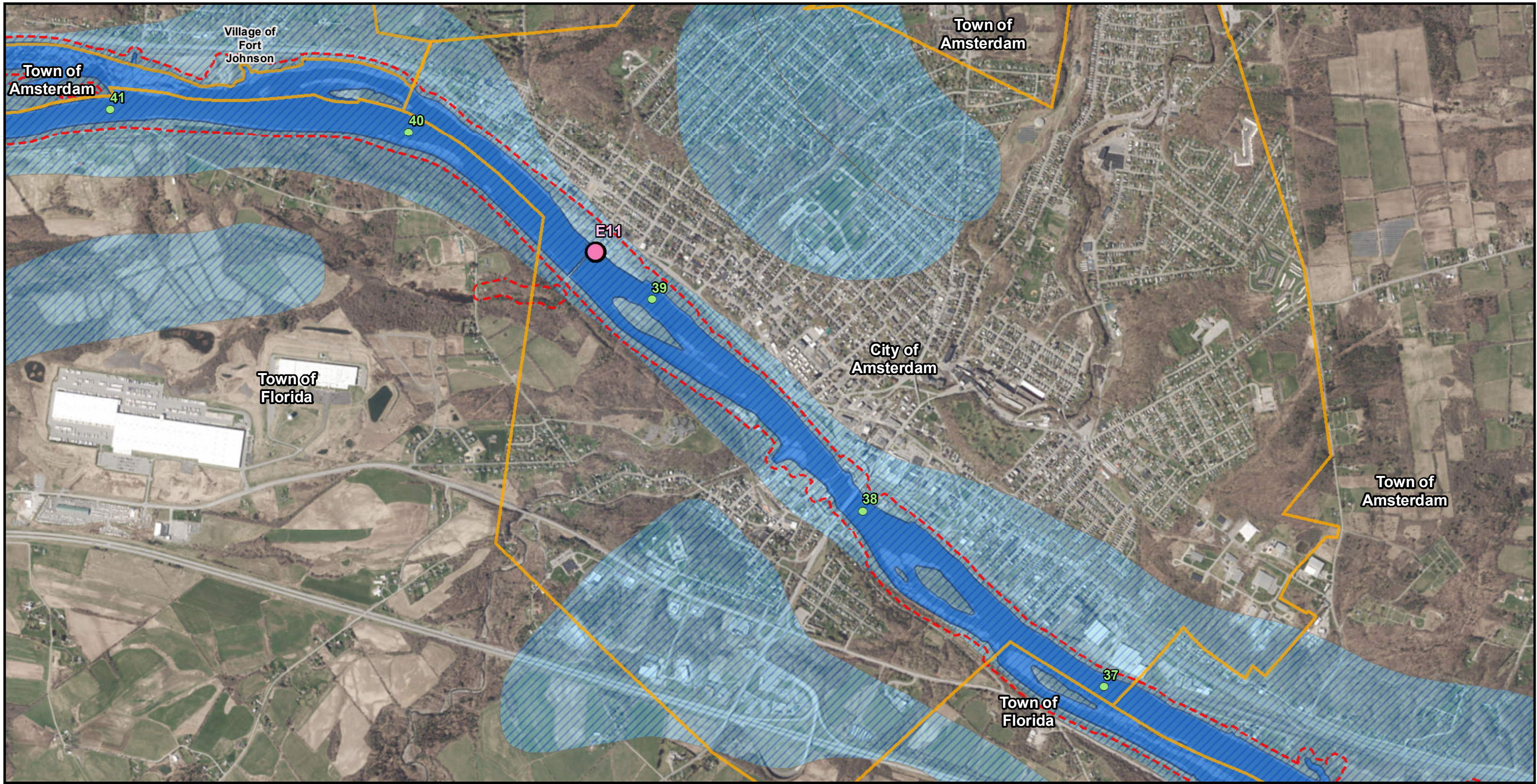
Figure 29F: Aquifers
